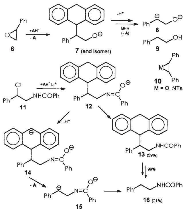
Scheme 3 Reactions of AH^- with benzylating agents 6 and 11 beginning with nucleophilic substitution followed by deprotonation of intermediates 7 and 12 and subsequent heterolytic BFR to benzyl anions 8 and 15 .
